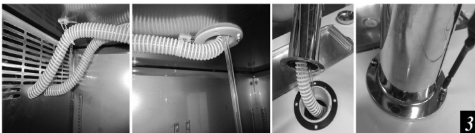
3. Insert air hose into the beer tower and secure beer tower to cabinet with the gasket under the beer tower.
