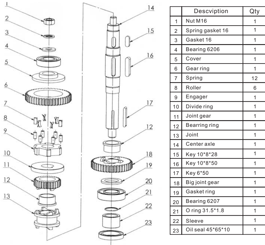
FIGURE 1 Center axle
