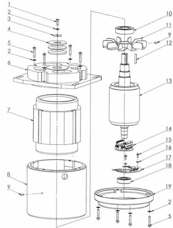
FIGURE 4 Motor
